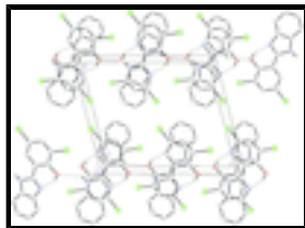
Fig. 2. The crystal packing of the title compound, viewed along the b -axis. The O-H...N and N-H...O hydrogen bonds are shown as dashed lines (see Table 1 for details).
